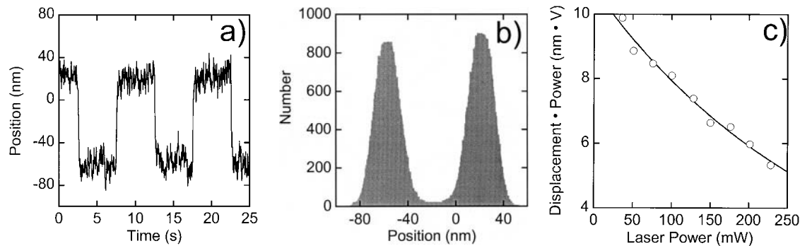
FIGURE 5 ( a ) Position time trace of a 502-nm-diameter polystyrene bead in glycerol when periodically moving the sample back and forth at 0.1 Hz with constant speed 910 nm/s. ( b ) Position histogram of the time trace in a . ( c ) Laser-power dependence of the product of laser power and displacement out of the laser trap as determined from histograms as in b . Circles represent the data, the line represents a fit of the data by Eq. 5.
